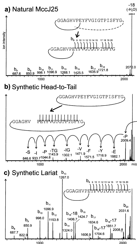
Figure 2. Comparison of MALDI-ion trap MS 2 spectra obtained from (a) natural MccJ25 and the synthetic microcin-isomers (b) 3 and (c) 4. In each case, the parent ion at m/z 2107.0 is selected and fragmented using identical instrument settings. The arrows in spectrum (b) indicate sequential residue losses.
